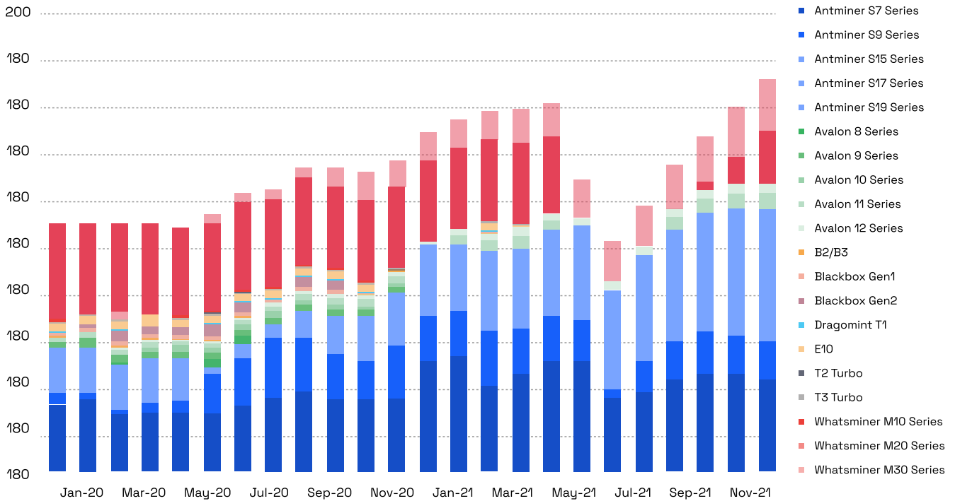
Figure 3: Total Hashrate by Hardware Unit (EH/s)
